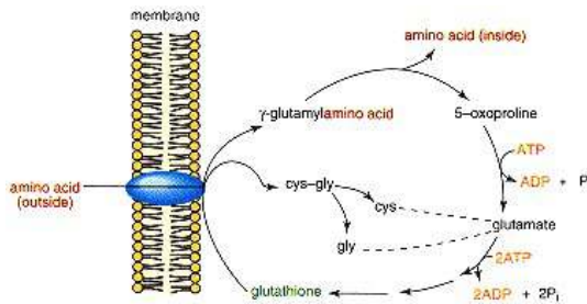
Figure 11.83 \gamma -Glutamyl cycle for transporting amino acids.
