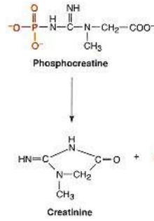
Figure 11.79 Spontaneous reaction forming creatinine.
