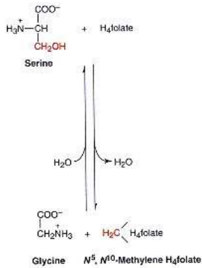
Figure 11.38 Serine hydroxymethyltransferase.
