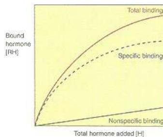
Figure 20.26 Typical plot showing specific hormone binding.
