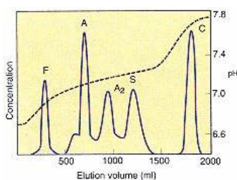
Figure 2.57 Example of ion-exchange chromatography. Elution diagram of an artificial mixture of hemoglobins F, A, A 2 , S, and C on carboxymethyl–Sephadex C-50. From Dozy, A. M., and Juisman, T. H. J. J. Chromatog. 40:62, 1969.
