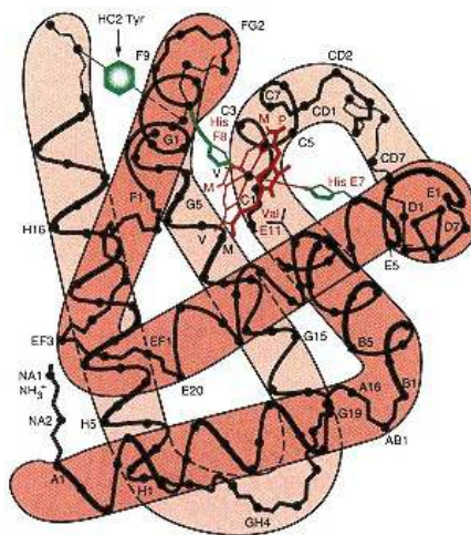
Figure 3.33 Secondary and tertiary structure characteristics of chains of hemoglobin. Proximal His F8, distal His E7, and Val E11 side chains are shown. Other amino acids of polypeptide chain are represented by -carbon positions only; the letters M, V, and P refer to the methyl, vinyl, and propionate side chains of the heme. Reprinted with permission from Perutz, M. Br. Med. Bull. 32: 195, 1976.
