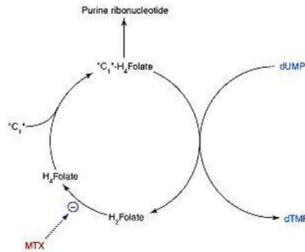
Figure 12.39 Relationships between H 2 folate, de novo purine nucleotide synthesis, and dTMP synthesis.
