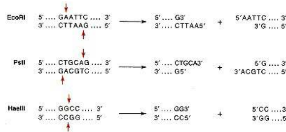
Figure 14.47 Types of products generated by type II restriction endonucleases. Enzymes exemplified by EcoRI and PstI nick on both sides of the center of symmetry of the palindrome, generating single-stranded stubs. Commonly used enzymes generate 5' ends, although some produce stubs with 3' ends as shown for PstI. Other restriction nucleases cut across the center of symmetry of the recognition sequence, producing flush or blunt ends, as exemplified by HaeIII.
