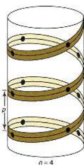
Figure 2.25 The helix pitch ( p ) for a helix with n = 4 . Each circle on a line represents an \alpha -carbon from an amino acid residue. The rise per residue would be p/n (see equation in text). From Dickerson, R. E., and Geis, I. The Structure and Action of Proteins . Menlo Park, CA: Benjamin, 1969, p. 26.
