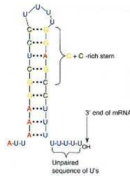
Figure 16.15 The stem-loop structure of the RNA transcript that determines rho-independent transcriptional termination. Note the two components of the structure: the G + C-rich stem and loop, followed by a sequence of U residues.
