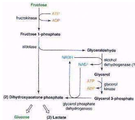
Figure 7.42 Pathway of glucose formation from fructose, along with the competing pathway of fructolysis.
