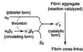
Figure 22.48 Activation of transglutaminase by thrombin.
