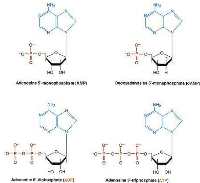
Figure 12.3 Adenosine nucleotides.
