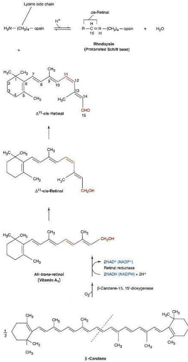
Figure 22.20 Formation of 11-cis-retinal and rhodopsin from \beta -carotene.
