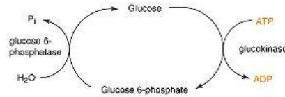
Figure 7.15 Phosphorylation of glucose followed by dephosphorylation constitutes a futile cycle in parenchymal cells of the liver.
