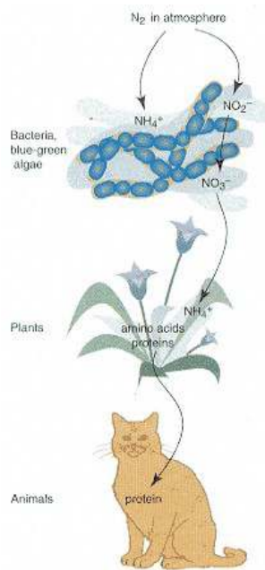
Figure 11.1 Outline of entry of atmospheric nitrogen into the human diet. This occurs initially by reduction of nitrogen to ammonia by enzymes in microorganisms and plants.
