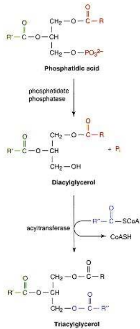
Figure 9.17 Synthesis of triacylglycerol from phosphatidic acid.
