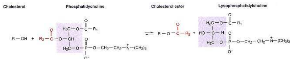
Figure 10.39 Lecithin:cholesterol acyltransferase (LCAT) reaction, where R—OH indicates cholesterol.
