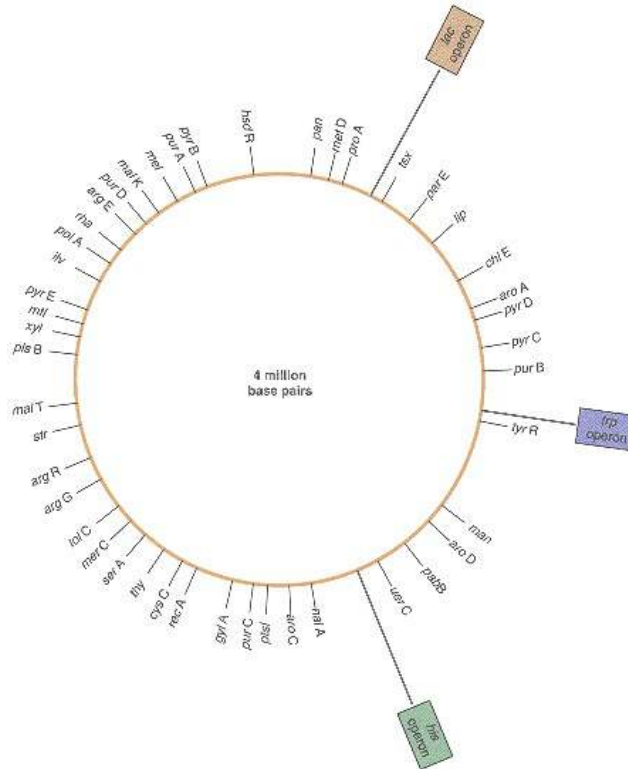
Figure 19.1 Partial genetic map of E. coli . The locations of only a few of the genes identified and mapped in E. coli are shown here. Three operons discussed in this chapter are indicated. Reproduced with permission from Stent, G. S., and Calendar, R. Molecular Genetics, An Introductory Narrative . San Francisco: Freeman, 1978, p. 289; modified from Bachmann, B. J., Low, K. B., and Taylor, A. L. Bacteriol Rev. 40:116, 1976.
