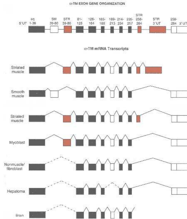
Figure 16.27 Alternate splicing of tropomyosin gene transcripts results in a family of tissue-specific tropomyosin proteins.
