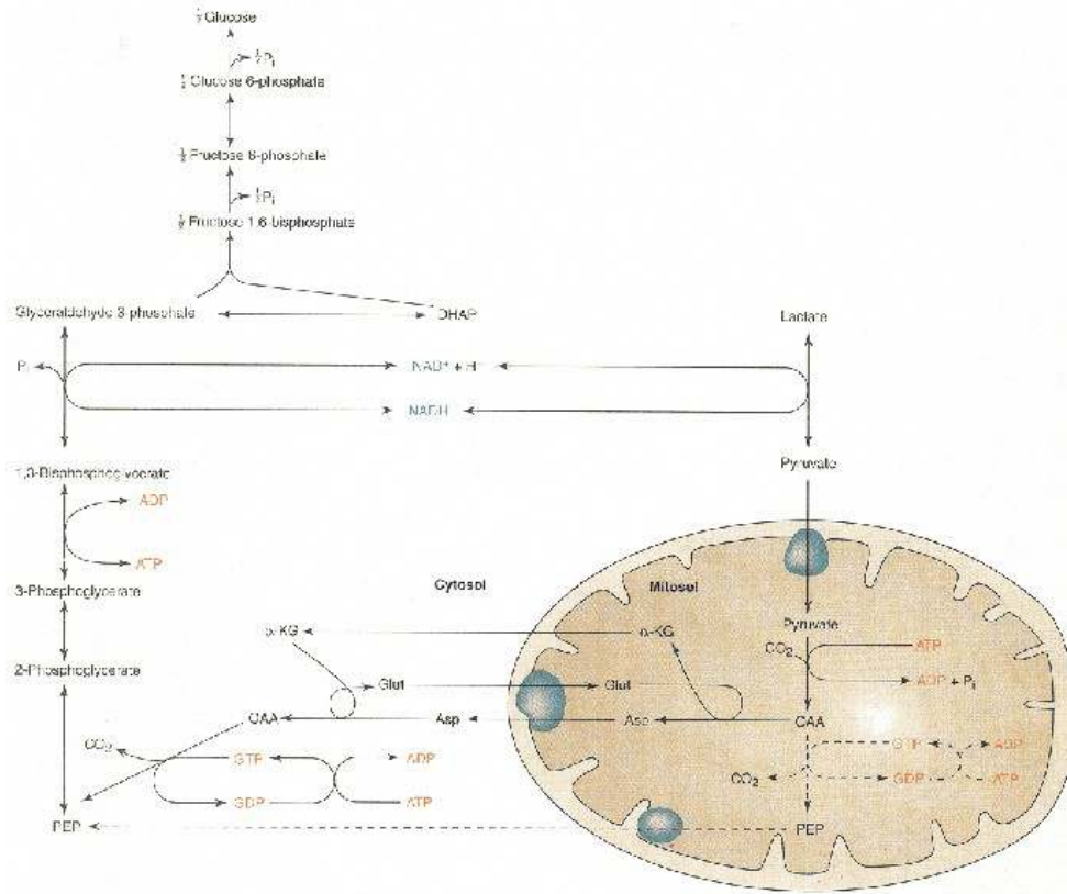
Figure 7.33 Pathway of gluconeogenesis from lactate. The involvement of the mitochondrion in the process is indicated. Dashed arrows refer to an alternate route, which employs mitosomal PEP carboxykinase rather than the cytosolic isoenzyme. Abbreviations: OAA, oxaloacetate; -KG, -ketoglutarate; PEP, phosphoenolpyruvate; DHAP, dihydroxyacetone phosphate.
