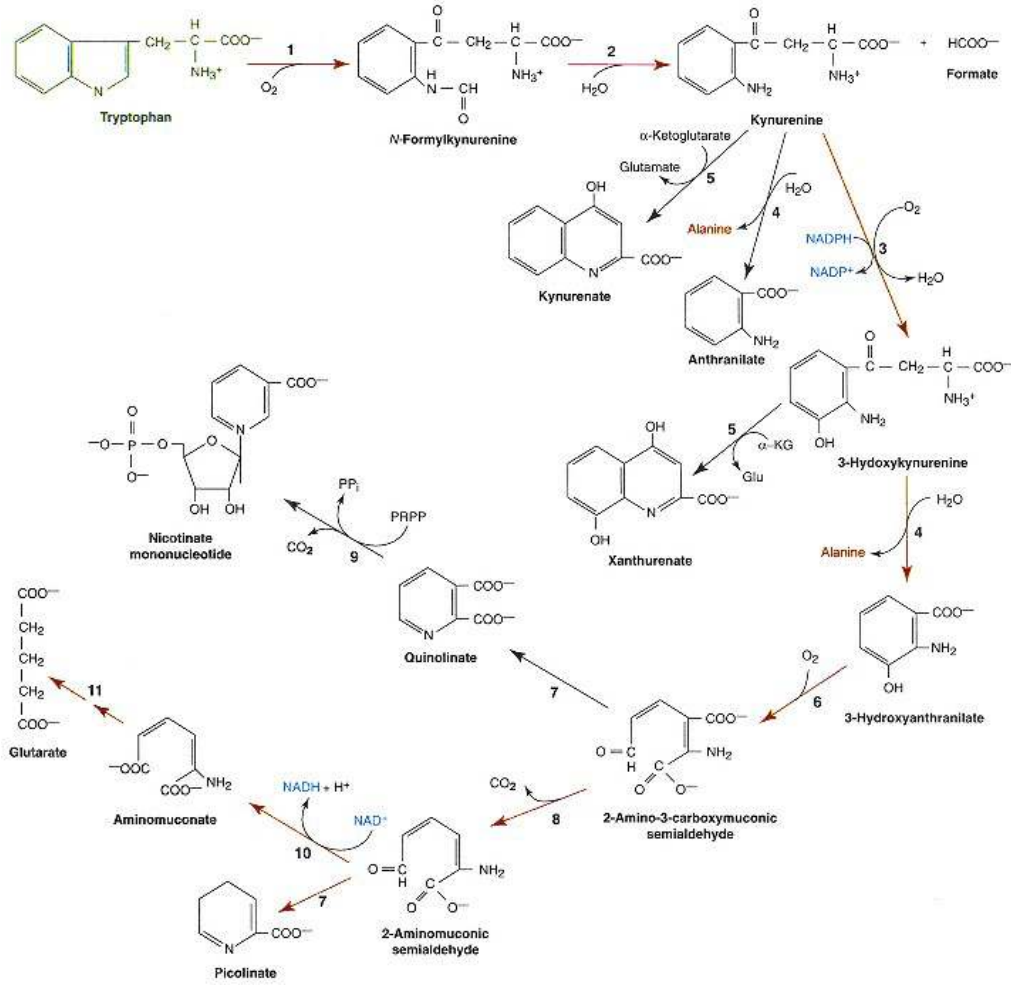
Figure 11.66 Metabolism of tryptophan. Major pathway is shown in red. Enzymes indicated by number are (1) tryptophan oxygenase, (2) kynurenine formamidase, (3) kynurenine hydroxylase, (4) kynureninase, (5) aminotransferase, (6) 3-hydroxyanthranilate oxidase, (7) spontaneous nonenzymatic reaction, (8) picolinate carboxylase, (9) quinolinate phosphoribosyltransferase, (10) aldehyde dehydrogenase, and (11) complex series of reactions.
