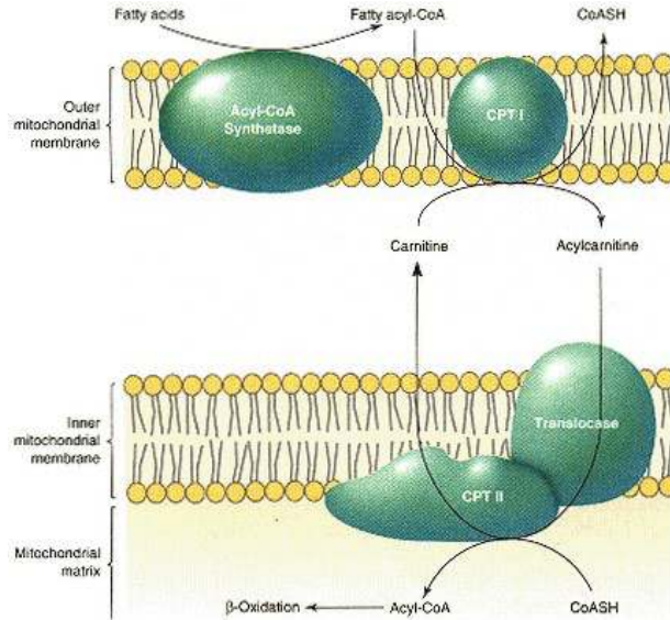
Figure 9.19 Mechanism for transfer of fatty acids from the cytosol through the inner mitochondrial membrane for oxidation.
