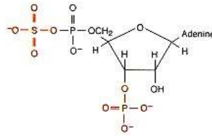
Figure 10.56 Structure of PAPS (3-phosphoadenosine 5-phosphosulfate).
