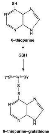
Figure 11.81 Conjugation of a drug by glutathione transferase.
