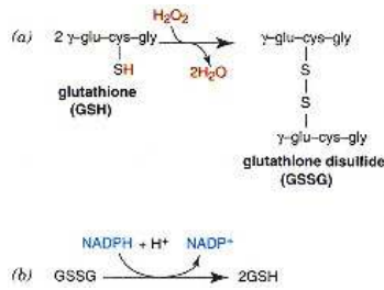
Figure 11.80 (a) Scavenging of peroxide by glutathione peroxidase and (b) regeneration of reduced glutathione by glutathione reductase.
