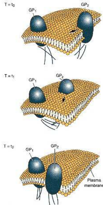
Figure 5.27 Modified version of the fluid mosaic model of biological membranes to indicate the mobility of membrane proteins.
