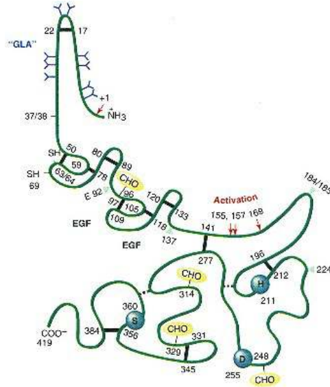
Figure 3.14 Schematic of domain structure for protein C showing multi-domain structure. "GLA" refers to the \gamma -carboxyglutamic residues (indicated by tree structures) in the NH_2 -terminal domain, disulfide bridges are indicated by thick bars, EGF indicates positions of epidermal growth factor-like domains, and CHO indicates positions where sugar residues are joined to the polypeptide chain. Proteolytic cleavage sites leading to catalytic activation are shown by arrows. Amino acid sequence is numbered from NH_2 -terminal end, and catalytic sites of serine, histidine, and aspartate are shown by circled one-letter abbreviations S, H, and D, respectively. Redrawn from a figure in Long, G. L. J. Cell. Biochem. 33:185, 1987.
