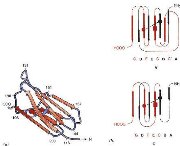
Figure 3.4 Immunoglobulin fold.
