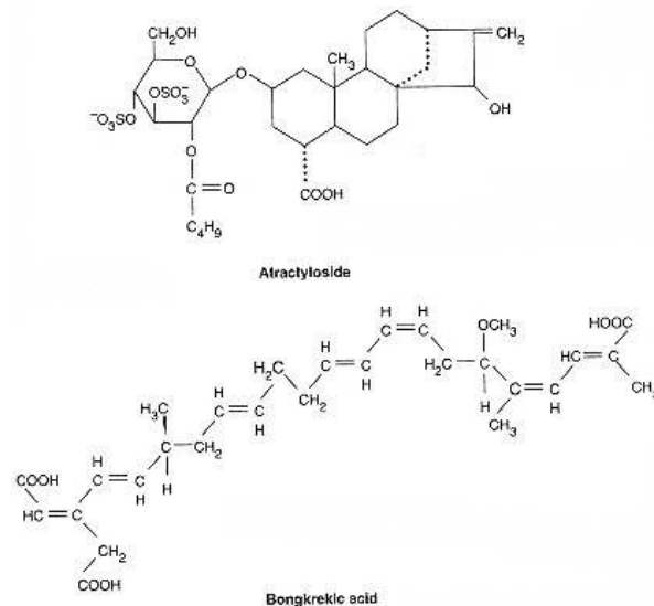
Figure 5.40 Structure of two inhibitors of the ATP–ADP transport system of liver mitochondria.
