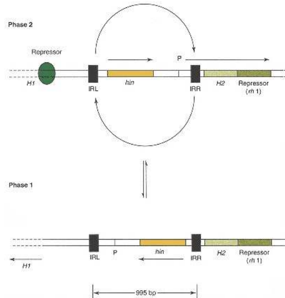
Figure 19.19 Organization of the flagellin genes of Salmonella . Orientation of a 995-bp DNA segment flanked by 14-bp inverted repeats (IRL and IRR) controls the expression of H1 and H2 flagellin genes. In phase 2, transcription initiates at promoter P within the invertible segment and continues through H2 and rh1 genes. In phase 1, the orientation is reversed so that transcription of H2 and rh1 genes does not occur.
