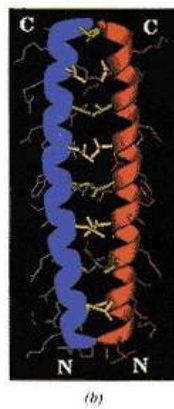
Figure 3.24 Leucine zipper motif of DNA-binding proteins.
