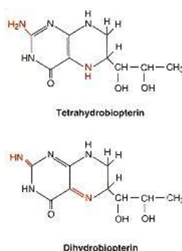
Figure 11.48 Biopterin.
