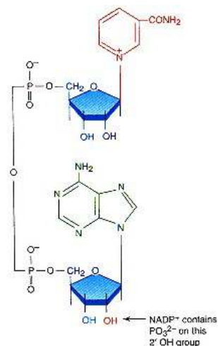
Figure 4.19 Nicotinamide adenine dinucleotide ( \text{NAD}^+ ).
