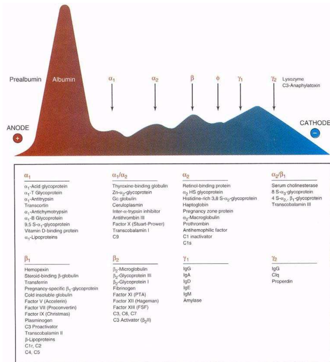
Figure 2.20 Electrophoresis pattern for plasma proteins at pH 8.6.
