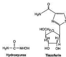
Figure 12.41 Structure of hydroxyurea and tiazofurin.
