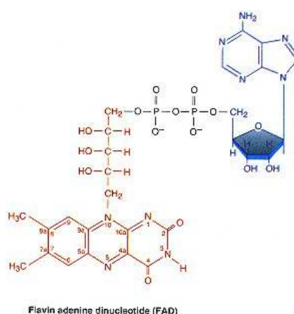
Figure 4.22 Flavin adenine dinucleotide (FAD).
