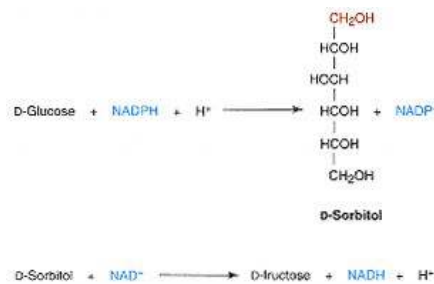
Figure 7.43 The pathway responsible for the formation of sorbitol and fructose from glucose.
