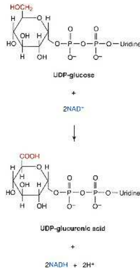
Figure 8.5 Formation of UDP-glucuronic acid from UDP-glucose.
