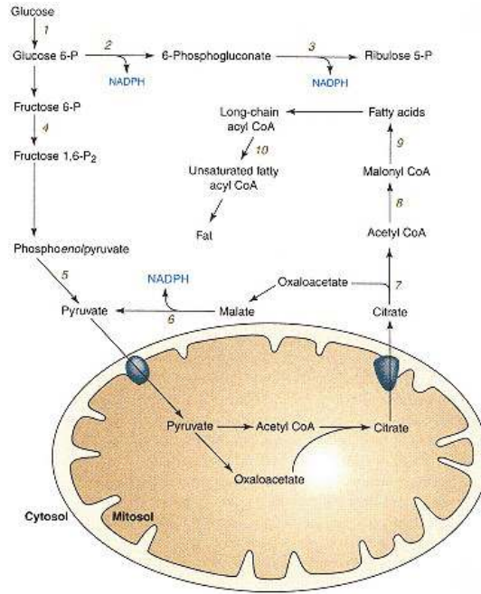
Figure 13.15 Enzymes induced in the liver of the well-fed individual.
