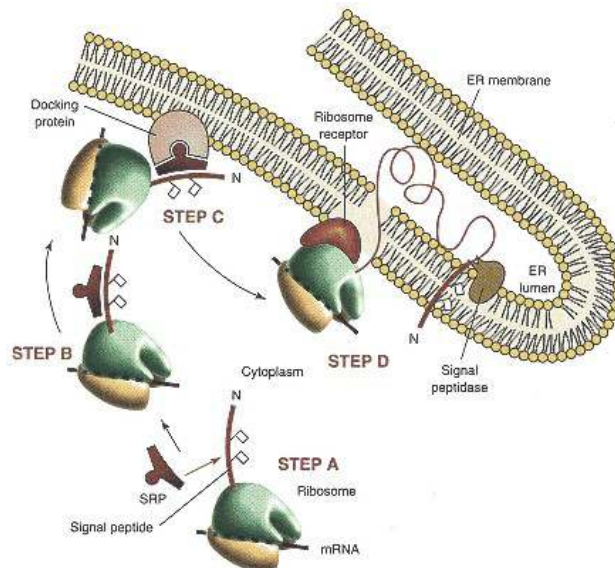
Figure 17.13 Secretory pathway: signal peptide recognition. At step A a hydrophobic signal peptide emerges from the exit site of a free ribosome in the cytosol. Signal recognition particle (SRP) recognizes and binds the peptide and peptide elongation is temporarily halted (step B). The ribosome moves to the ER membrane where docking protein binds to SRP (step C). In step D the ribosome is transferred to a ribosome receptor or translocon, protein biosynthesis is resumed, and newly synthesized protein is extruded through the membrane into the ER lumen.
