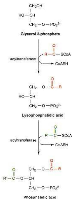
Figure 9.15 Synthesis of phosphatidic acid from glycerol 3-phosphate.
