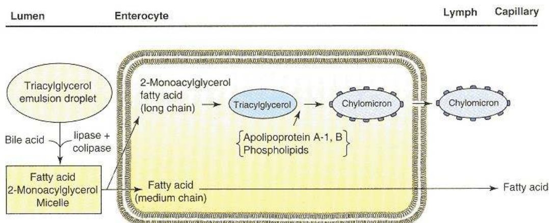
Figure 26.27 Digestion and absorption of lipids.
