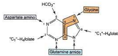
Figure 12.9 Sources of carbon and nitrogen atoms in the purine ring. C-4, C-5, and N-7 are from glycine; N-3 and N-9 from glutamine; C-2 and C-8 from "C 1 '"- H_4 folate; N-1 from aspartate; and C-6 from CO_2 .
