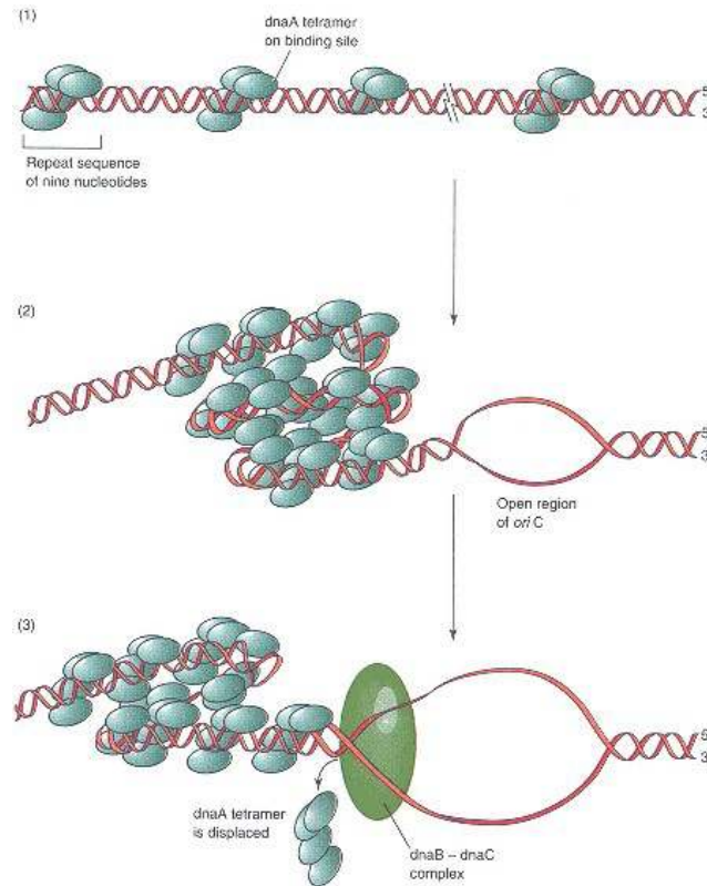
Figure 15.31 Model for initiation of replication in E. coli .
