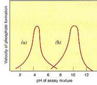
Figure 4.59 The pH dependence of (a) acid and (b) alkaline phosphatase reactions.
