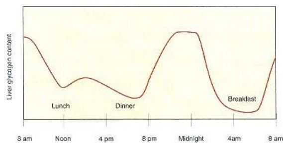
Figure 7.47 Variation of liver glycogen levels between meals and during the nocturnal fast.
