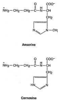
Figure 11.77 Anserine and carnosine.
